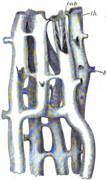
FIG. 152.— Syringopora , a fossil, showing autothecal tubes ( th ), funnel-shaped tabulae ( tab ), and tubular cross-bars ( t ).
